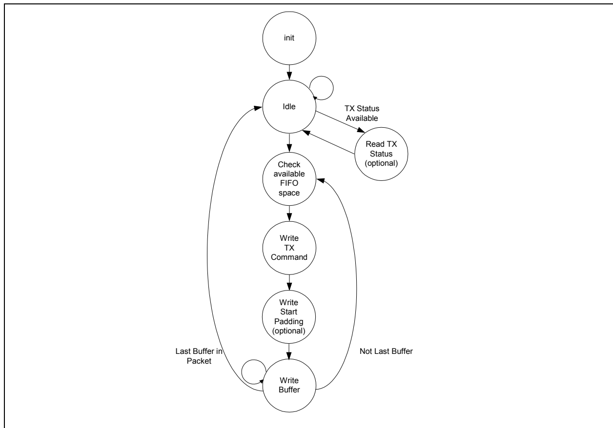
FIGURE 3-20: SIMPLIFIED HOST TX FLOW DIAGRAM
